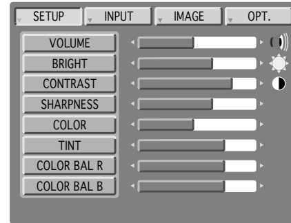
Figure 4.5 Video Signal
