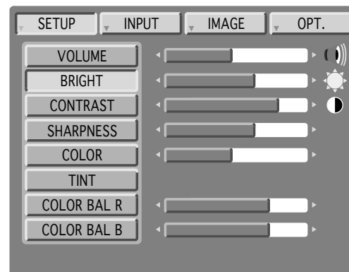
Figure 4.3 Default Settings
