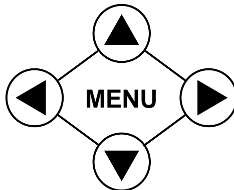
Figure 4.2 Menu Button
